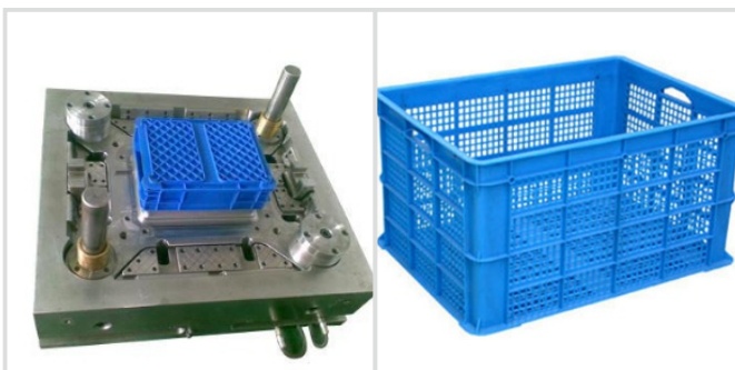
Plastic box injection mold and injection products
